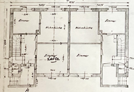
A Erdgeschoß
